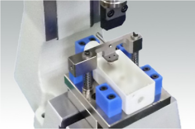
Spring pin press-fit
