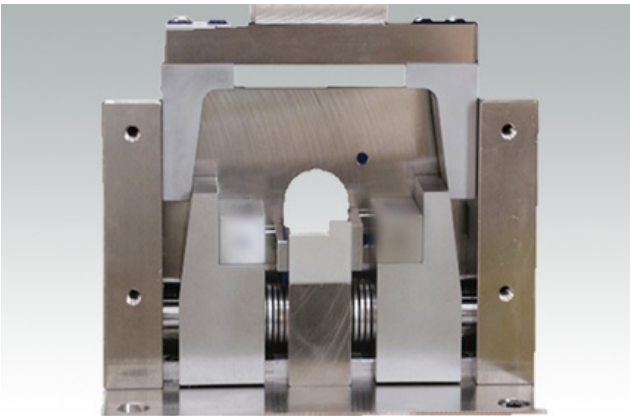
Punching process (motor terminal)
